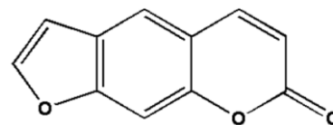
Fig 9 Chemical structure of Psoralen
