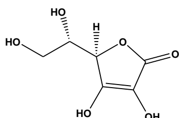
Fig 7 Structures of Vitamin C
