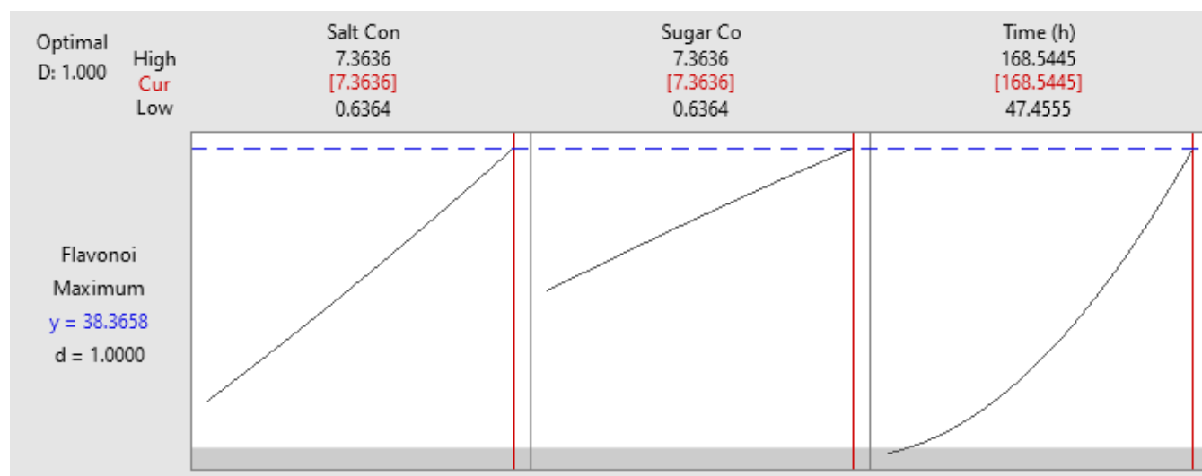
Figure 2: Response optimization plot of salt concentration, sugar concentration and fermentation time to get the highest flavonoid content of fermented climbing swamp fern.
